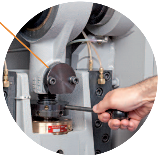
Quick adjustment of the clear height
